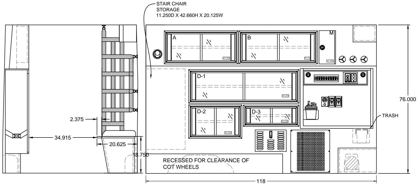
INTERIOR CABINET DIMENSIONS IN INCHES
