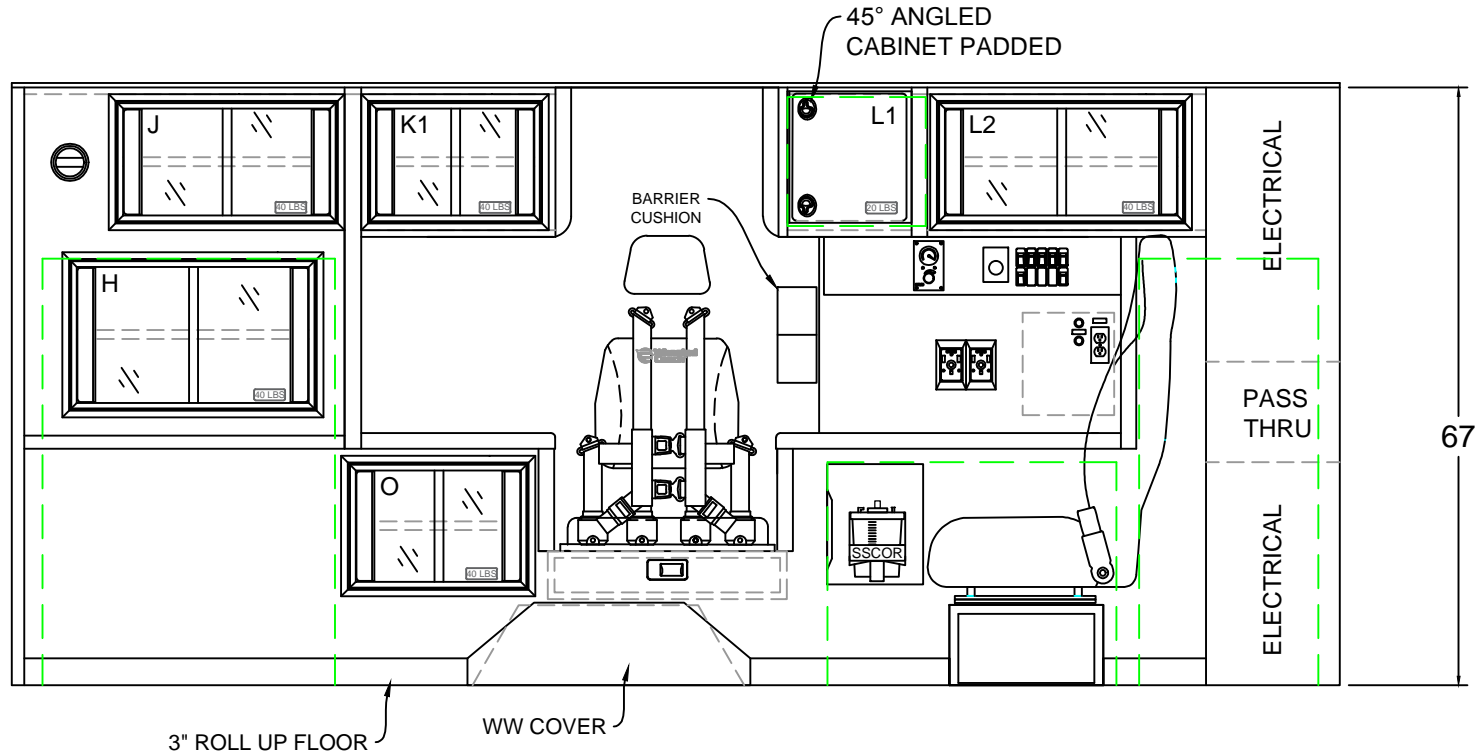
INTERIOR CABINET DIMENSIONS IN INCHES
